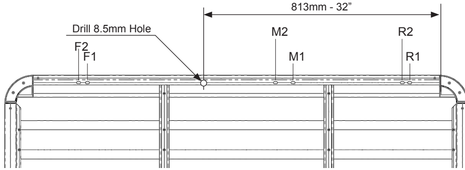
Front of Tray
