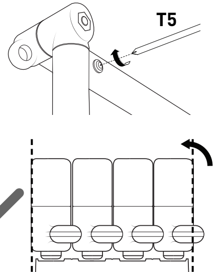
Fig. B: Loosen the screw behind the drop down hinge, adjust the arm rotation and re-tighten the screw.
